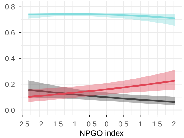
(j) NPGO index, 3-year ONDJFM mean
